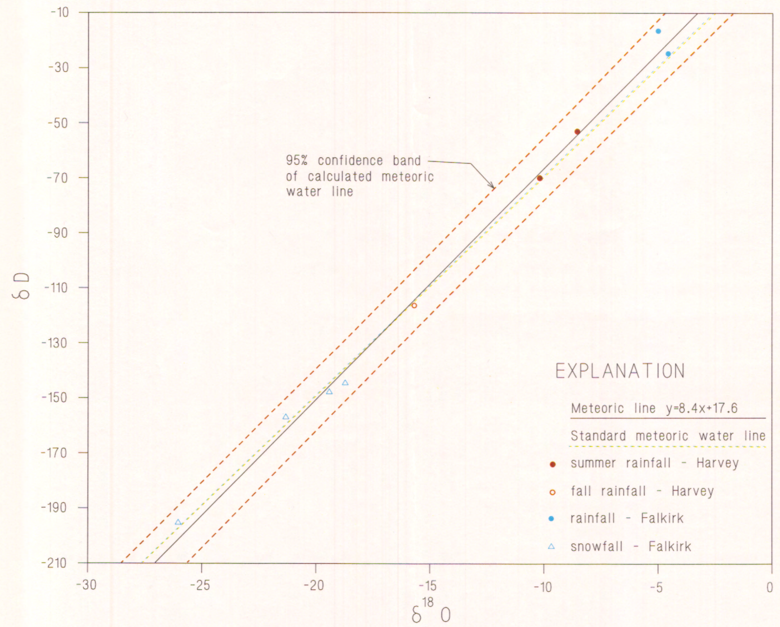
FIGURE 29. Meteoric water line determination from precipitation samples.
